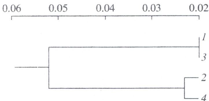
Fig. 2. Dendrogram of Cavalli-Sforza and Edwards genetic distance for summer and fall runs of chum salmon in the Kamchatka River (27 loci): 1 — summer run, 1989; 2 — fall run, 1990; 3 — summer run, 1991; 4 — fall run, 1991
